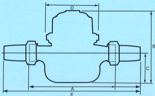
15mm-25mm Dimensions
