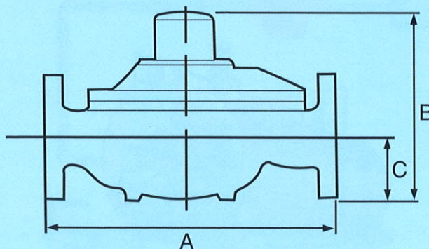
40mm-80mm Dimensions
